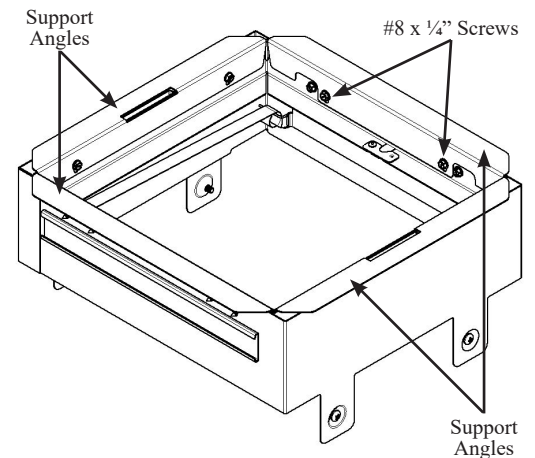
Fig. 4 - Support Angles Installation
