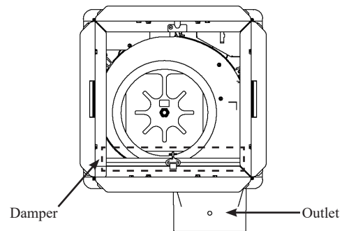
Fig. 7 - Damper Installation Direction
