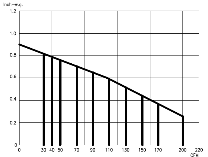
PQ Curve with pre-filter & MERV 13 filter
