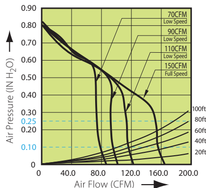
SMT150-200LED Fan Curve
