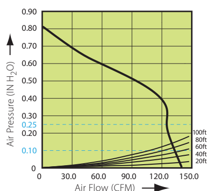
SMT130 Fan Curve
