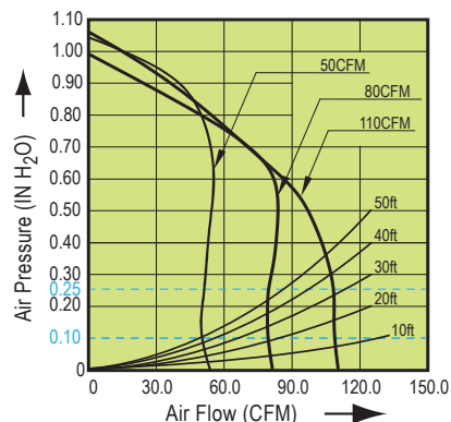
SLM80-110H-C Fan Curve
